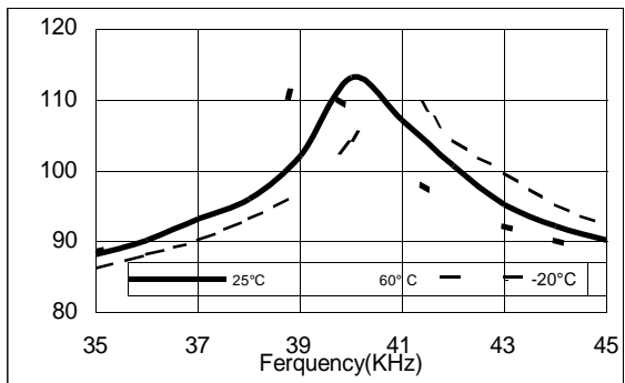
Temperature Characteristic
