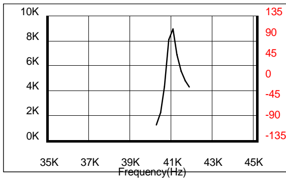
Sound Pressure Level VS Frequency
