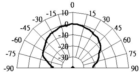
Directivity
