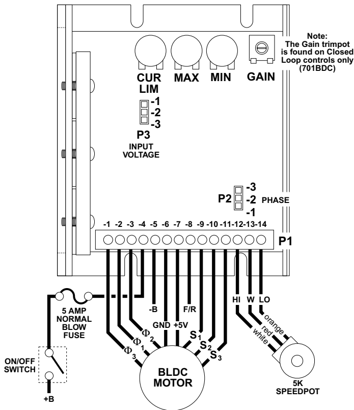
STANDARD HOOK-UP WIRING DIAGRAM
