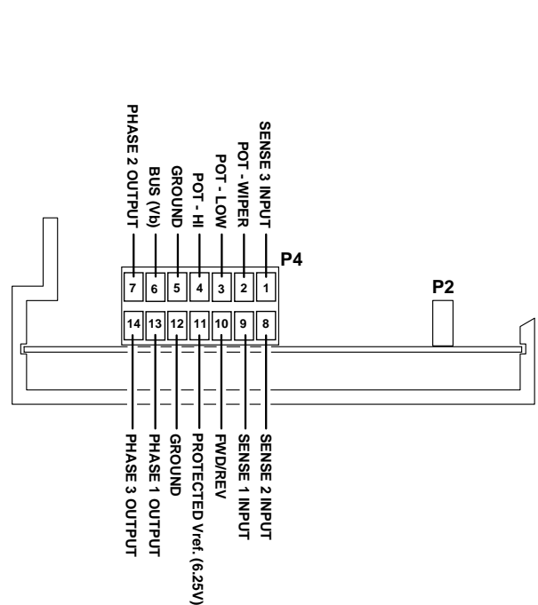
-PA OPTION HOOK-UP WIRING DIAGRAM
