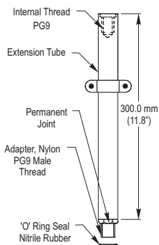
Extension Assembly
