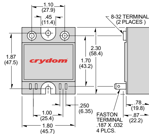
All dimensions are in inches (millimeters)
