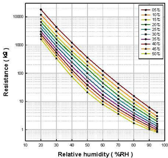
Fig. 3. Temperature characteristics
