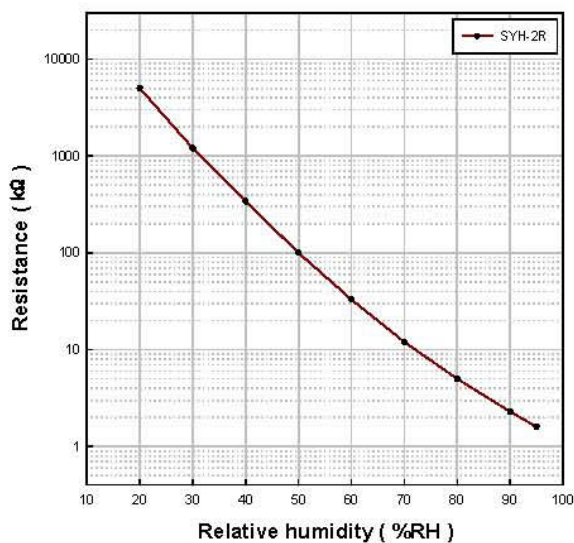
Fig. 2. Standard characteristics
