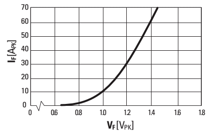
Fig. 1: On-state current versus on-state voltage (instantaneous values)
