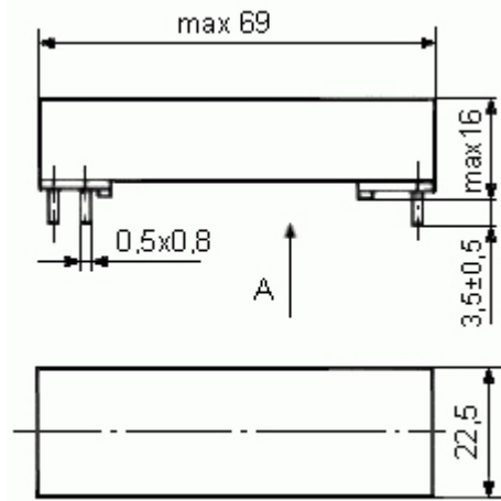
View from the bottom side of relay
